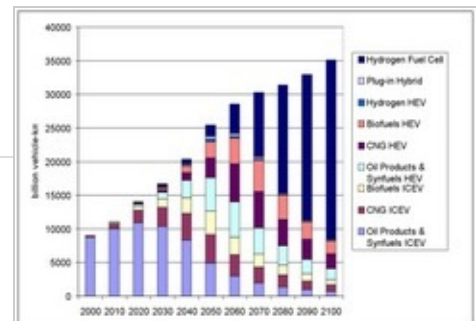
Development of personal transport scenarios across different climate change mitigation scenarios (from top: 650 ppmv, 450 ppmv).
